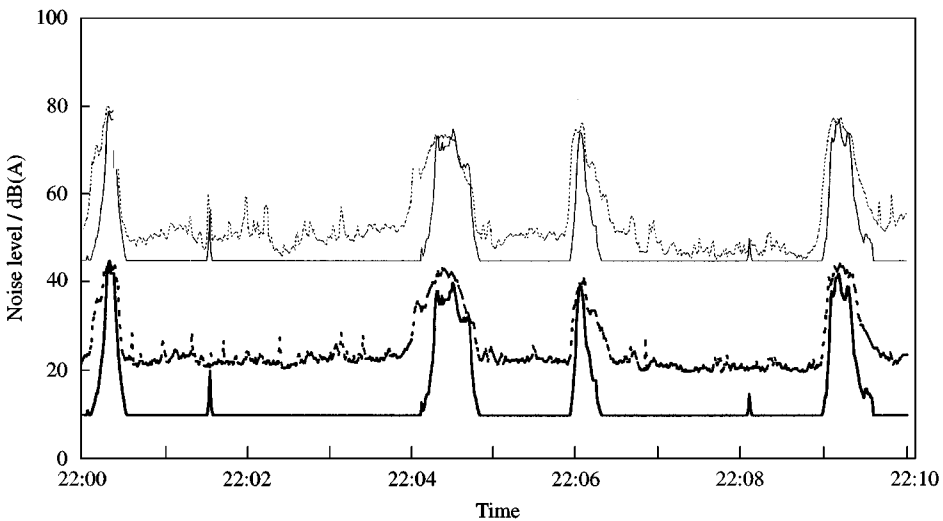
Figure 1. Example of short-time measurements and noise-time pattern outdoor and indoor calculated from continuous measurements: \cdots , outdoor measurement; \text{—} , calculated outdoor noise level; \text{---} , indoor measurement; \text{—} , calculated indoor noise level.
